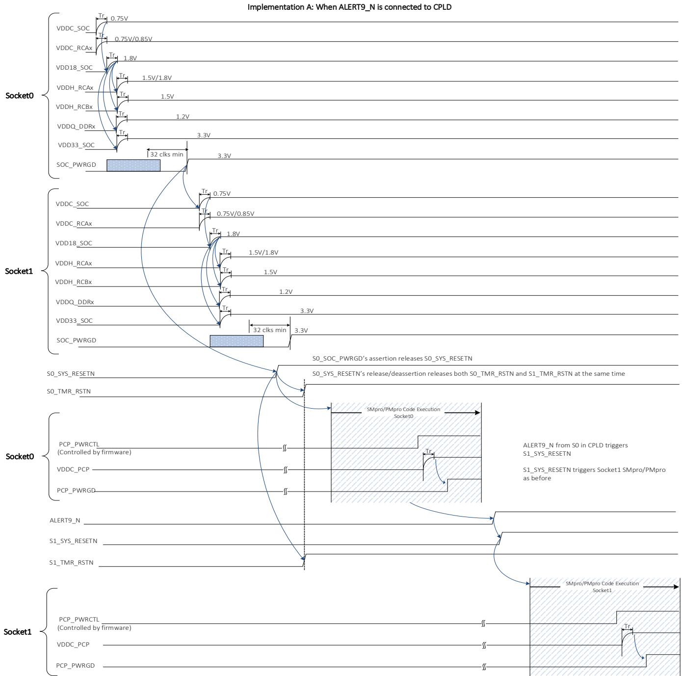
Figure 8: Power-on Sequence for 2P Configuration when ALERT9_N is Connected to CPLD
