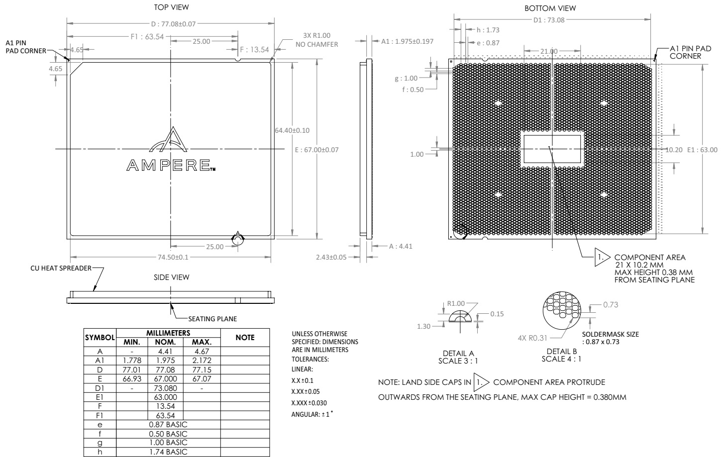
Figure 1: Altra Max 77.080 mm × 67.000 mm 4926-Pin Flip Chip Land Grid Array (FCLGA) Mechanical Data
