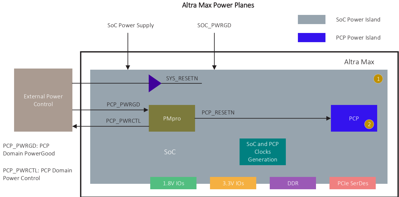
Figure 3: Connecting Altra Max to an External Power Device
