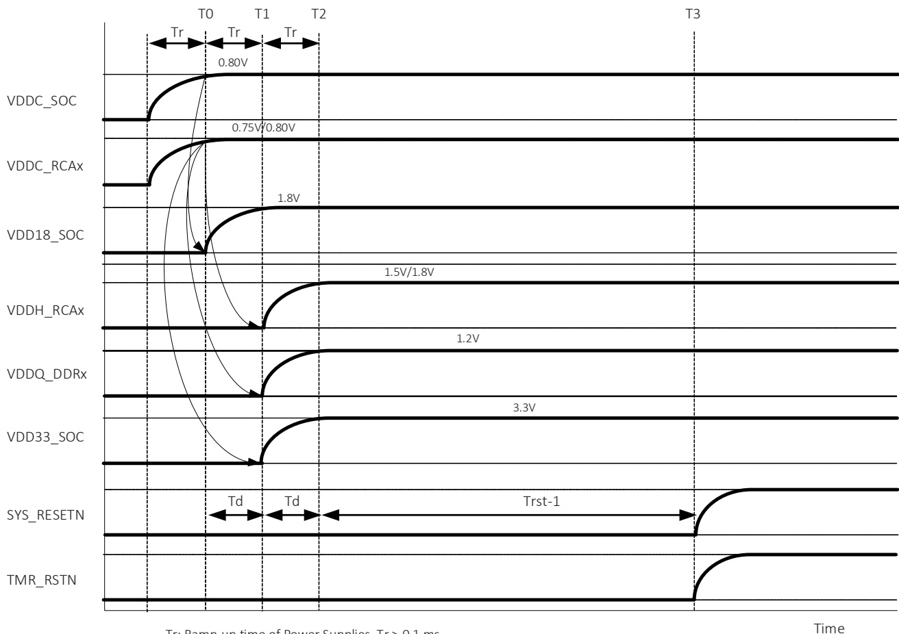
Figure 4: Power-on Voltage Sequencing – SoC Domain
